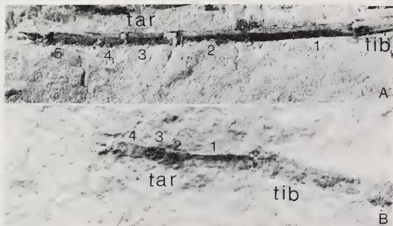
Figure 13. Photographs of tarsi of Protereismatidae and Misthodotidae: A, Protereisma permianum , MCZ 3402, Permian of Kansas. Length of tarsus, 8 mm. B, Misthodotes obtusus , MCZ 3402, Permian of Kansas. Length of tarsus, 1.5 mm. TIB, tibia; TAR, tarsus.
